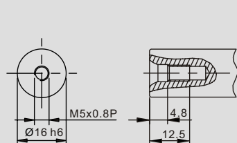
Shaft Option S1
