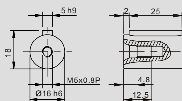
Shaft Option S2
